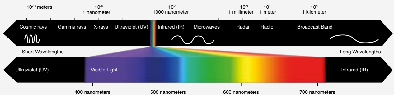
Figure 6.29 The light spectrum.
