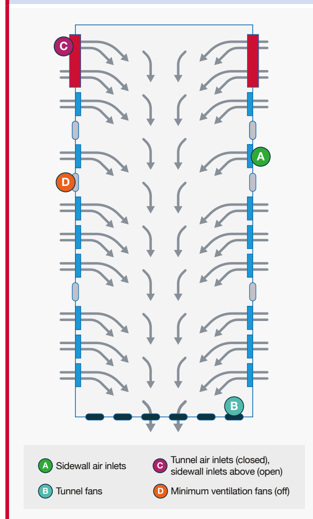
Figure 6.16 Typical air movement during transitional ventilation.
